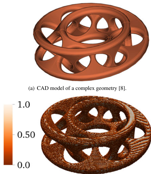
(b) Volume fractions of the geometry within the mesh volume elements of an overlaid 200 x 100 x 200 Cartesian mesh.
