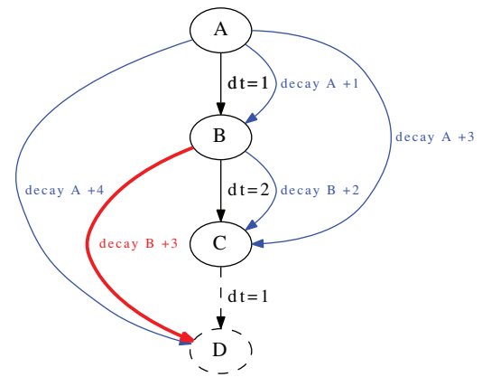
Fig. 4. A simple decay line cache holding compositions A, B, C, and a yet-uncomputed composition D. B comes from decaying A 1 time step. C comes from decaying B 2 time steps, etc. Black represents the cache for this particular composition chain. Blue indicates decay operations that can be satisfied by cache lookups. If A needs to be decayed 1 time step (A +1), a quick lookup returns the previously computed B. Decaying B 3 time steps requires a decay calculation to compute a new composition D, but subsequent requests such as decaying A 4 time steps will not require any recalculation.
