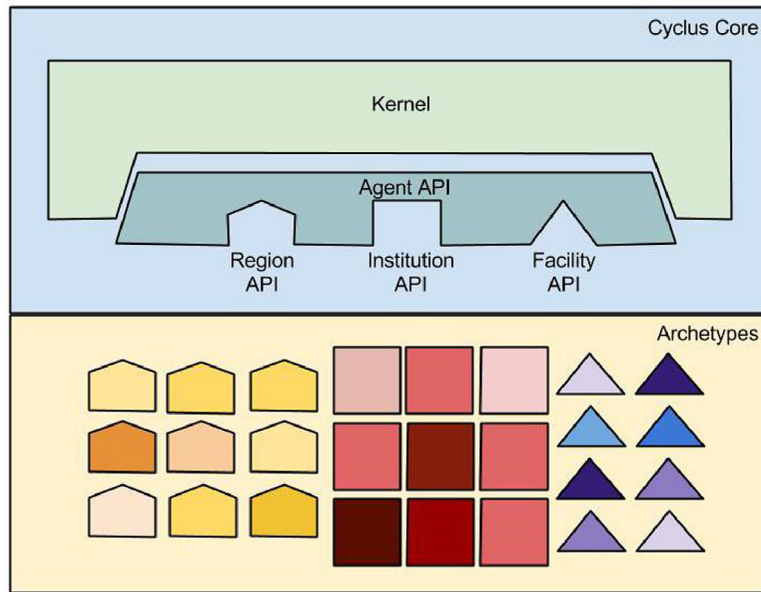
Fig. 1. The CYCLUS core provides APIs that abstract away the details in the kernel and allow the archetypes to be loaded into the simulation in a modular fashion.
