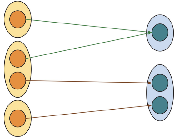
Fig. 5. The flow graph representing three suppliers (left), two requesters (right), and the potential flows of various commodities among them. The second consumer makes two different requests. Meanwhile, the second supplier can supply the commodities requested by both consumers and has provided two bids accordingly [35].
