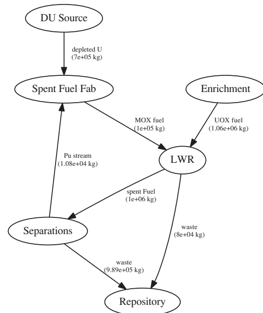
Fig. 6. 1-pass MOX recycle scenario material flows.
