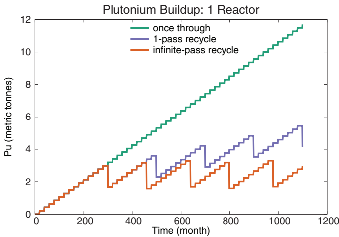
Fig. 8. System plutonium buildup with one reactor.
