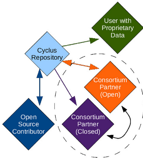
Fig. 2. The CYCLUS framework enables fully open, partially open, and fully closed collaborations [36].
