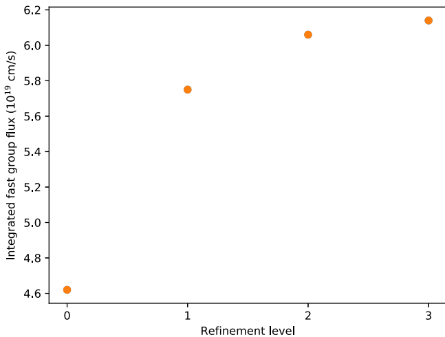
Fig. 2. Plot of the integrated fast group flux as the mesh in isotropically refined.
