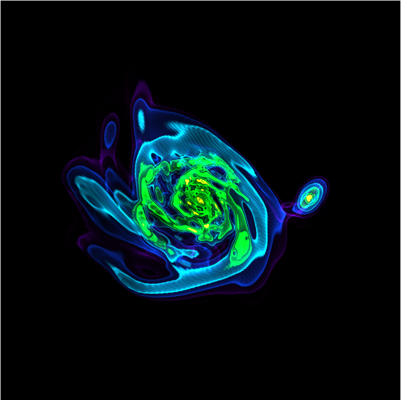
Figure 26: Volume rendering of gas density isocontours around a galaxy in a cosmological zoom-in simulation performed with RAMSES. Adapted from [104].
