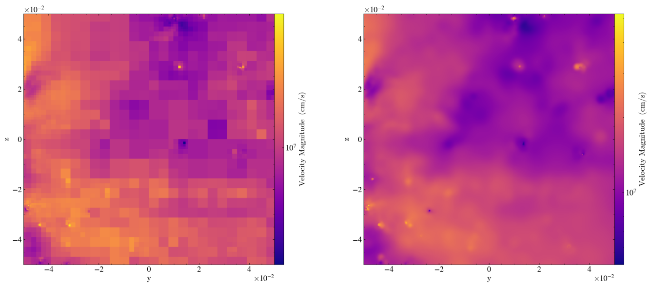
Figure 10: Comparisons between the older, octree-based method used in version 3.0 of yt (left) and the newer, “demeshed” algorithm used in yt 4.0 and beyond (right). The left image clearly shows artifacts from the octree structure imposed on the underlying dataset by yt , and the right hand side is much smoother, with more definition at individual pixels. The difference in color bars is notable as well, accounted for by the different normalization methods.
