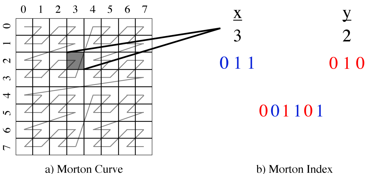
Figure 18: Example of 3rd order Morton curve in two dimensions. The bits of the x and y indices are interleaved to generate a single integer that fully describes the cell's location within the two-dimensional domain to within 1/2^3 th of the domain in each dimension.
