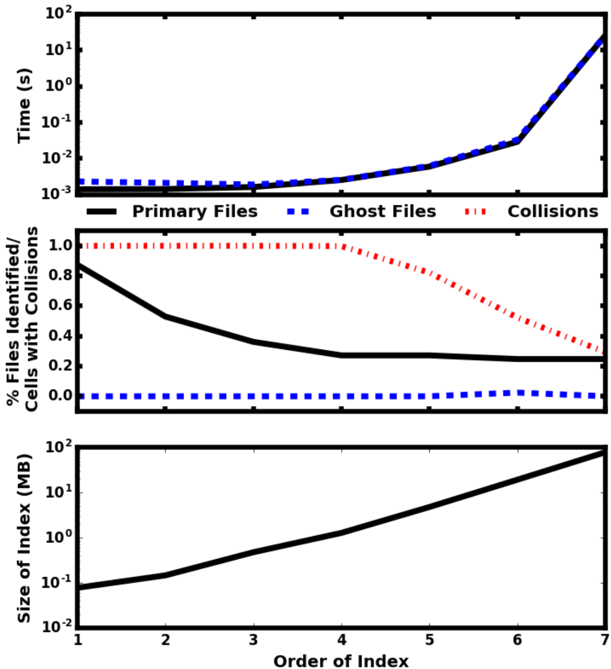
Figure 22: Dependence of query time (top), fraction of files selected/cells with collisions (middle), and index size (bottom) on the total refinement of the bitmap index. The solid black lines correspond to the query times and files identified by just the selectors. The dashed blue lines correspond to the query times and additional files selected when a ghost zone with the width of one Morton cell is added around the selectors. The dash-dotted line in the middle panel shows the fraction of cells with collisions between files. NOTE: maybe this would make more sense as scatter plots ? (connecting dots to fill a continuous yet unreachable space of non-integer-limited x values seems inappropriate.
