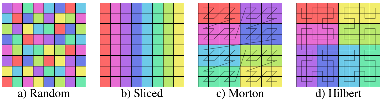
Figure 14: Examples of four different schemes for partitioning a 2D domain between 8 files. Each color represents a different file.
