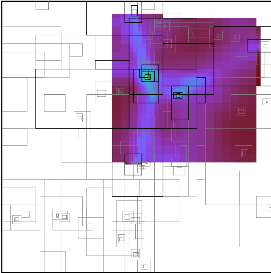
Figure 4: A selection of data in a low-resolution simulation from a rectangular prism.
