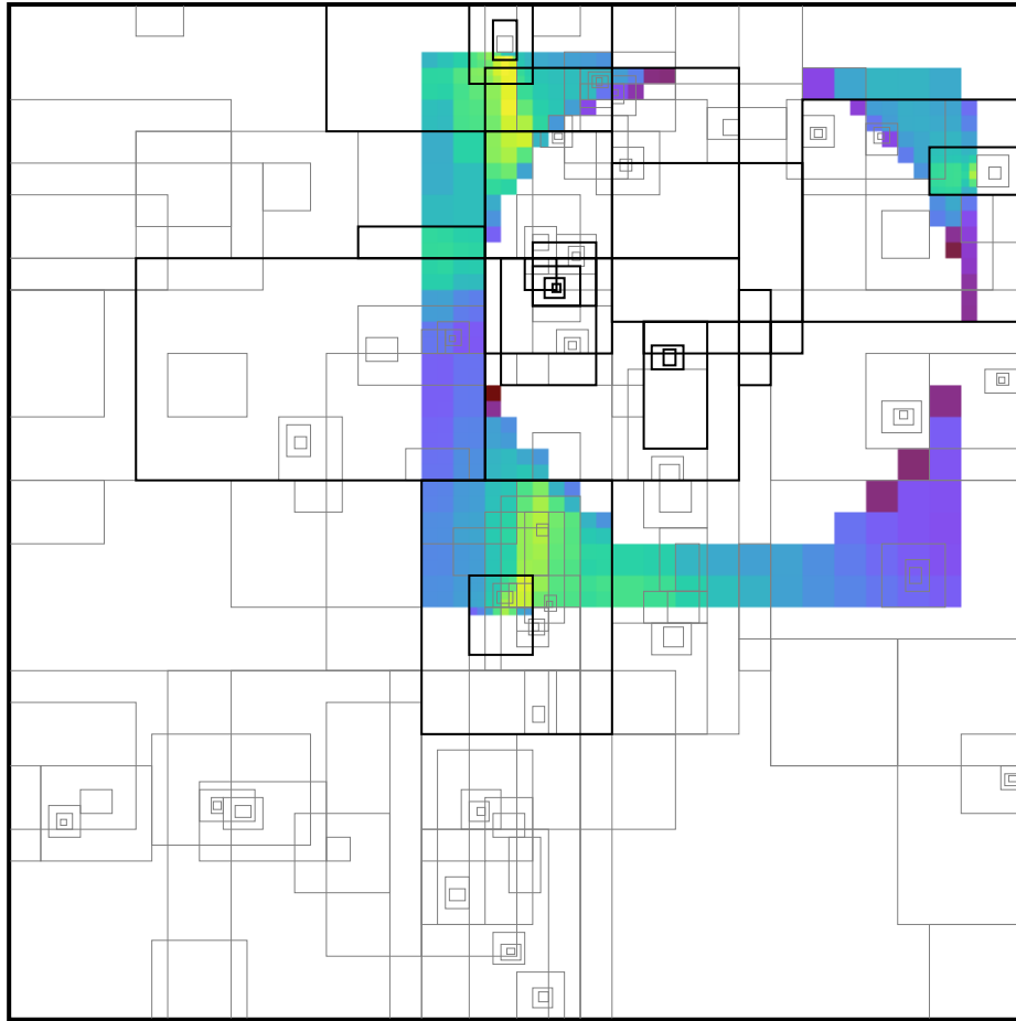
Figure 6: The logical A AND NOT B for regions A and B from Figures 4 and 5 respectively.
