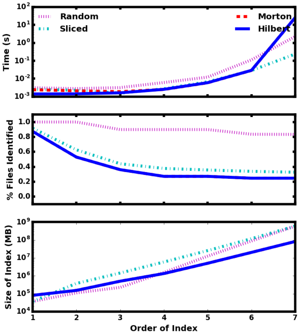
Figure 25: Dependence of query time (top), the number of files selected (middle), and the size of the index (bottom) on index order for different domain partitioning between files. The dotted magenta lines are for a randomly partitioned dataset, the cyan dashed-dotted lines are a dataset partitioned by equal slices along one dimension, the dashed red lines are a dataset partitioned along an 6th order Morton curve, and the solid blue lines are a dataset partitioned along a 6th order Hilbert curve. NOTE: it looks like the Morton curve is almost always behind the Hilbert one. Can you use zorder to put it at the frontrow instead so that we can see both ?
