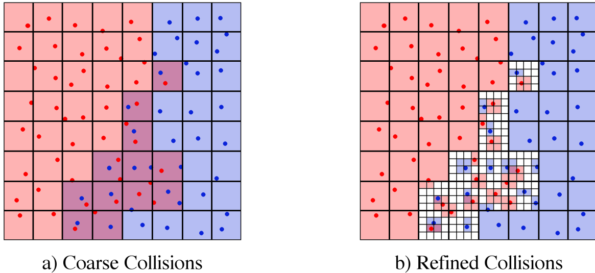
Figure 19: Examples of a collision between two files. The red points and blue points are contained by two different files. The larger grid in both panels denotes the boundaries of 3rd order Morton cells. The cells containing points from either file are shaded accordingly such that cells containing points from both files are purple. The smaller grids within these cells on the right are the boundaries of 2nd order Morton cells refining the collisions.
