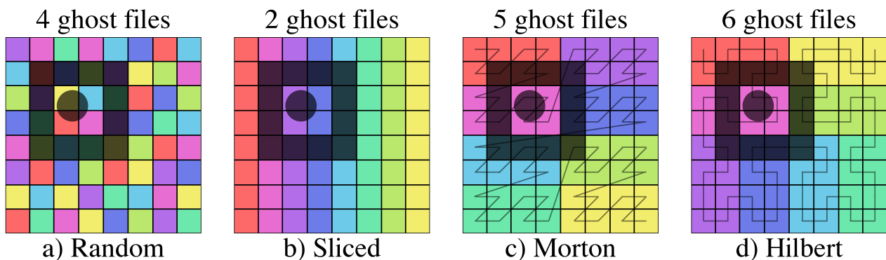
Figure 21: Examples of a selector ghost zone with a width of one Morton cell at an index order of 3 for four different domain partitioning schemes. The shaded circular region is the selector and the shaded box is the ghost zone. Different partitioning schemes will lead to different numbers of ghost files. NOTE: same as figure 13
