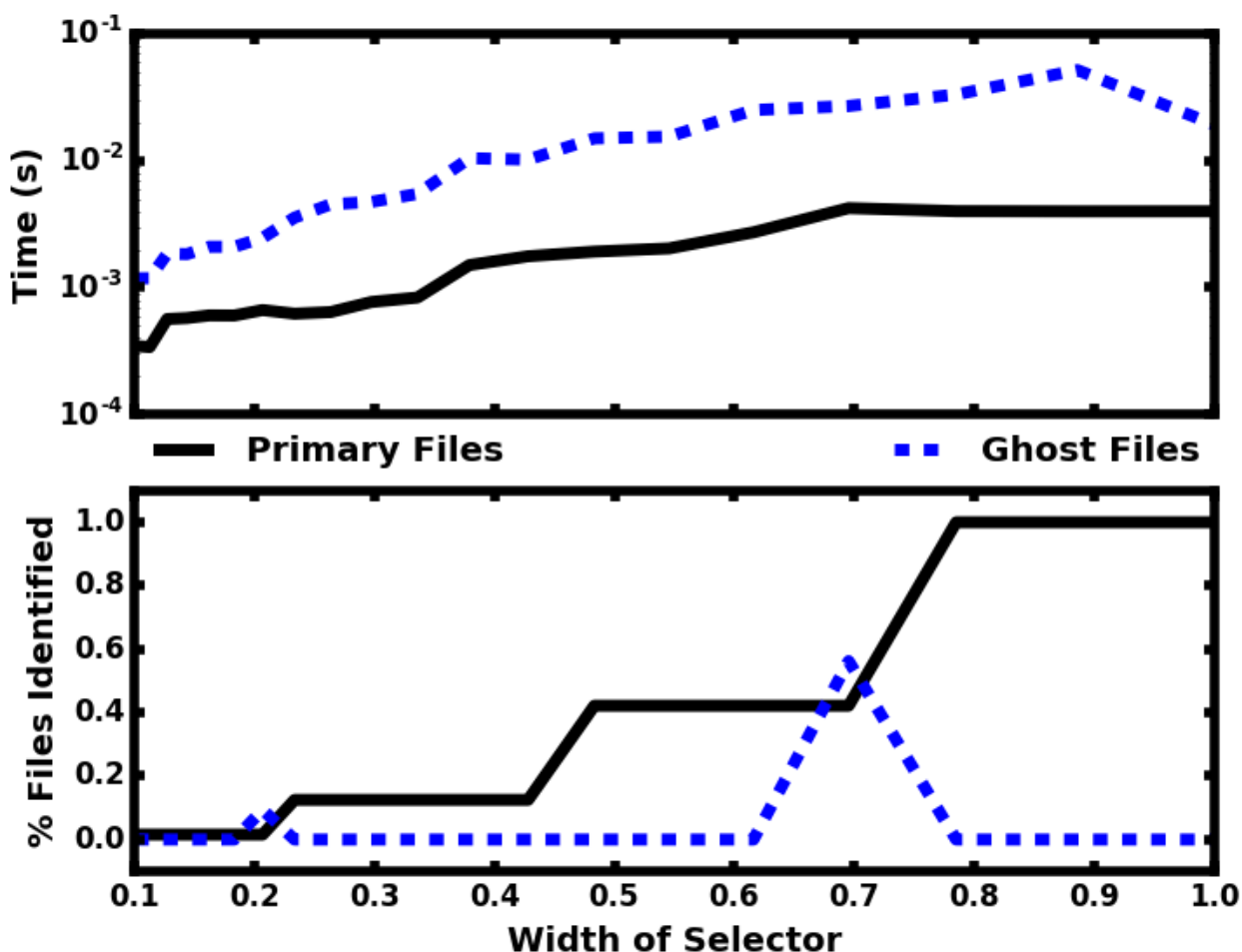
Figure 24: Dependence of query time (top) and number of files selected (bottom) on selector width in terms of the total domain width. The solid black lines correspond to the query times and files identified by the selectors alone. The dashed blue lines correspond to the query times and additional files identified when a ghost zone with a width of one cell is added to the selector.
