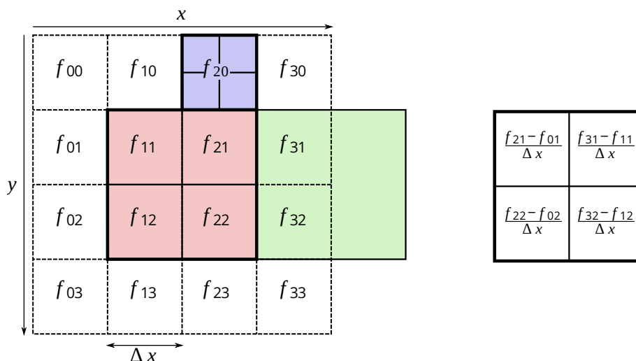
Figure 9: Scheme of the AMR structure used to estimate the gradient of a quantity in the central oct (red). Octs are represented in thick lines, cells in thin lines and virtual cells in dashed lines. Left panel: The virtual cell values on a 4^3 grid are interpolated from the nearest cell in the AMR grid. If the nearest cell is at the same (or coarser) level, its value is used directly. Note that virtual cells f_{31} and f_{32} have the value of the the actual coarser cell (green). If the cell is refined, the mean of its children is used (for example f_{20} is the mean of all the blue cells). Right panel: Gradients are estimated using a first-order finite difference centered scheme on the 4^3 virtual cells, here illustrated for a gradient along the x
