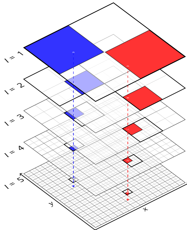
Figure 8: Illustration of a binary search through a quadtree. The search starts at the root level (level = 1 here) and recursively selects the quad that contains the point until reaching a leaf. The procedure is easily generalized in 3D.
