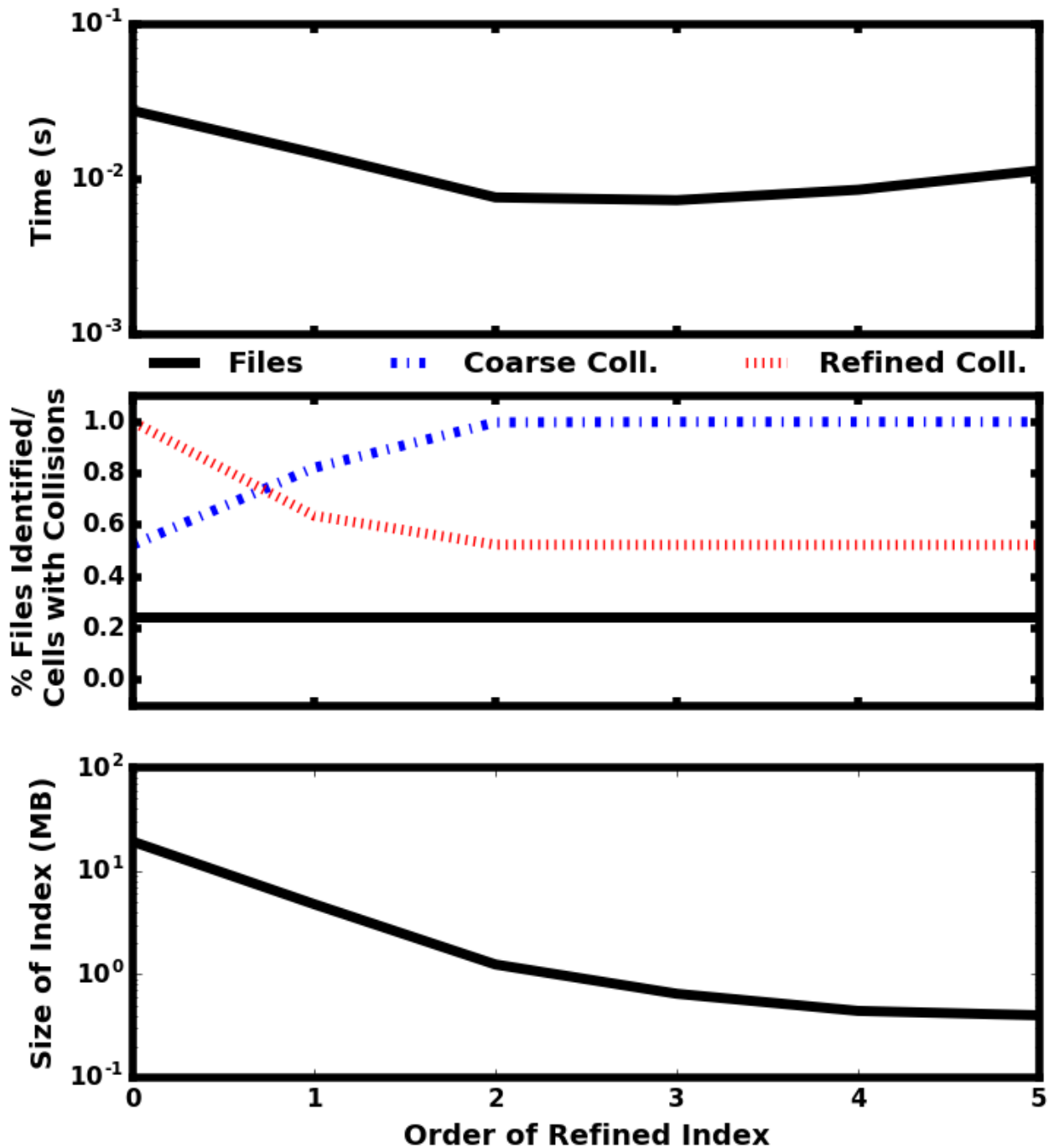
Figure 23: Dependence of query time (top), fraction of files selected/cells with collisions (middle), and memory required to store the index (bottom) on the order of the secondary index used to refine collisions. In the middle panel, the solid black line corresponds with the fraction of files identified, the dash-dotted blue line is the fraction of cells at the first index level that have collisions, and the dotted red line is the fraction of cells at the second index level that have collisions.
