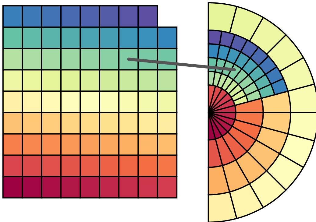
Figure 3: Index space to coordinate space mapping. On the left is an example of how data points may be laid out on disk and on the right is how these points might be translated into a (cylindrical) coordinate space.
