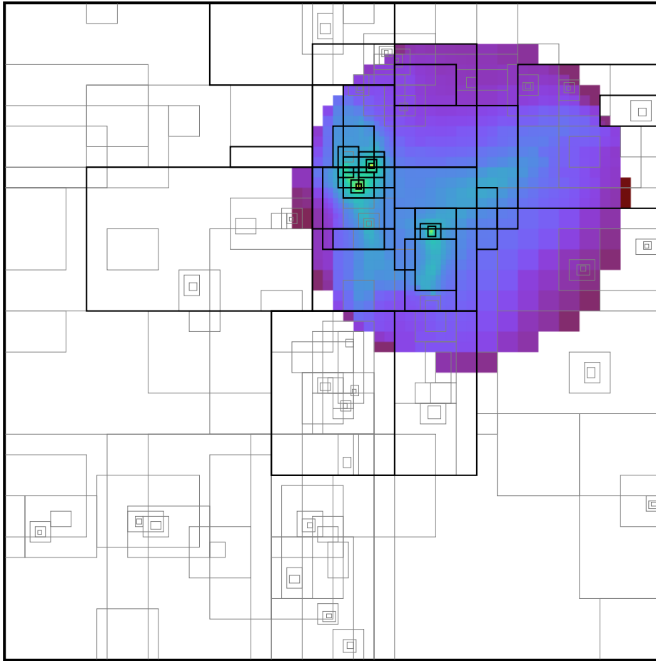
Figure 5: A selection of data in a low-resolution simulation from a sphere.
