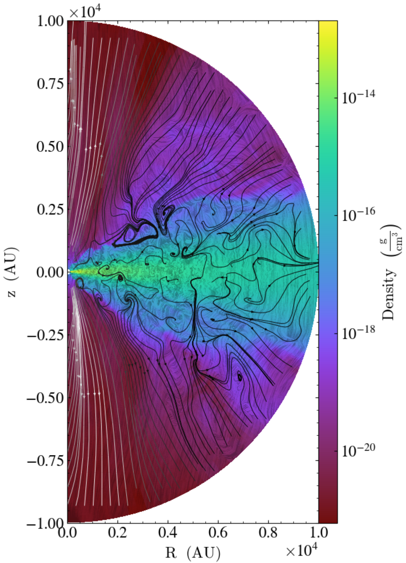
Figure 13: Spherical data from a protoplanetary disk, overlaid with annotations supplied by yt to demonstrate both the magnetic field and velocity structure of the data. Data are used, with permission, from a simulation based on the ones described in [12].
